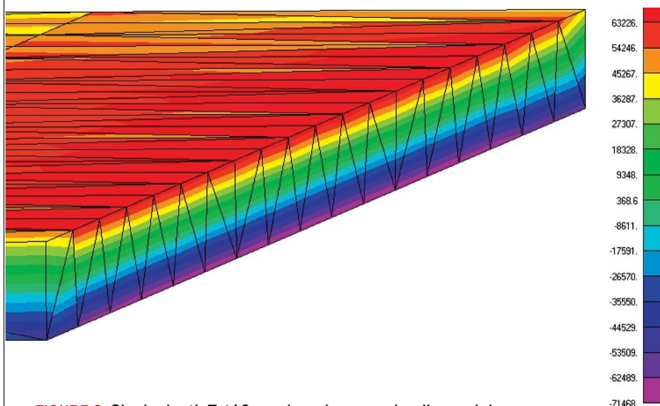
FIGURE 2: Single-depth Tet10 mesh under same loading, axial stresses.
