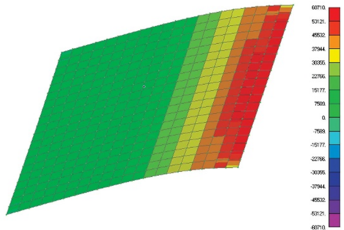
FIGURE 1: Top and bottom fiber stresses under bending.
