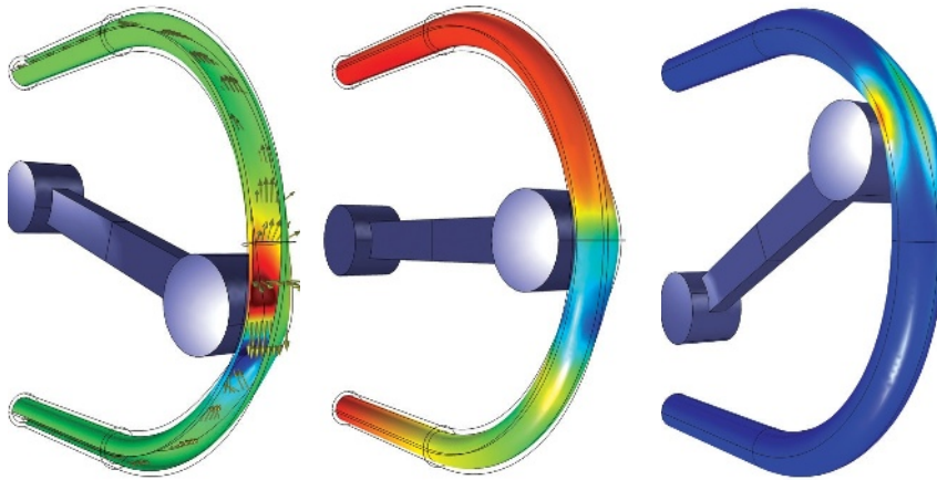
Flow, pressure and stress results from a COMSOL multiphysics fluid-flow analysis of a peristaltic pump for non-contact fluid flow control. The COMSOL analysis was done by Veryst Engineering. Images courtesy of Veryst Engineering.
