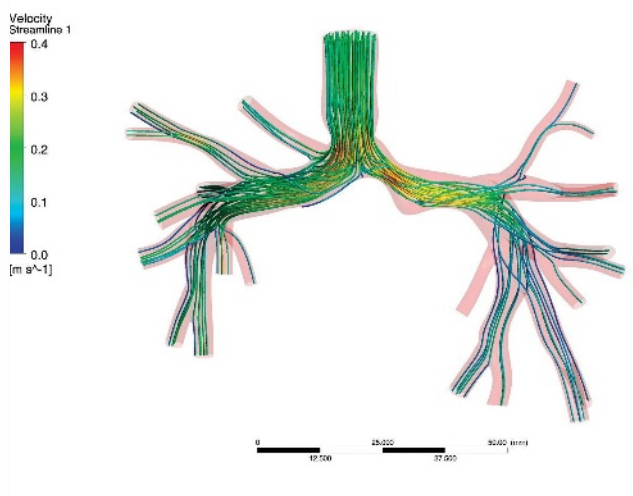
Pulmonary artery blood-flow simulation done in ANSYS Fluent CFD analysis software to evaluate surgical options. The goal is to increase blood flow to lungs in children born with only one functioning ventricle. Velocity pathlines simulate the injection of contrast medium in the superior vena cava to allow assessment of blood distribution from the upper body into pulmonary arteries. Image courtesy of ANSYS.
