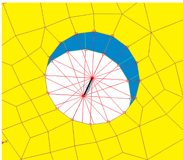
FIGURE 4: 1D/2D idealization of a bolted joint in a plate.
