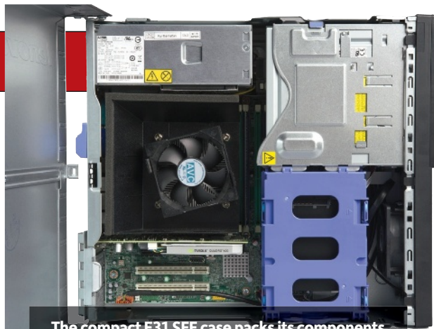
The compact E31 SFF case packs its components neatly into its small, but well organized interior.
